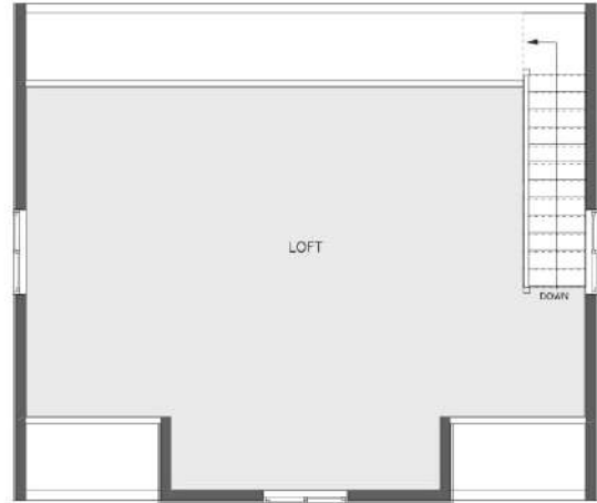
LOFT PLAN 482 SQ FT
